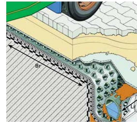
Figure 2. Effective roof area m 2 Lr = length of the roof to be drained (in metres) Br = the plan width of roof from gutter to ridge (in metres)
